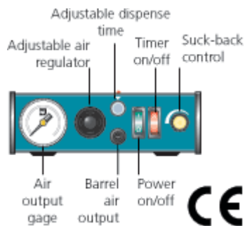
Front Panel of the JB1113N
